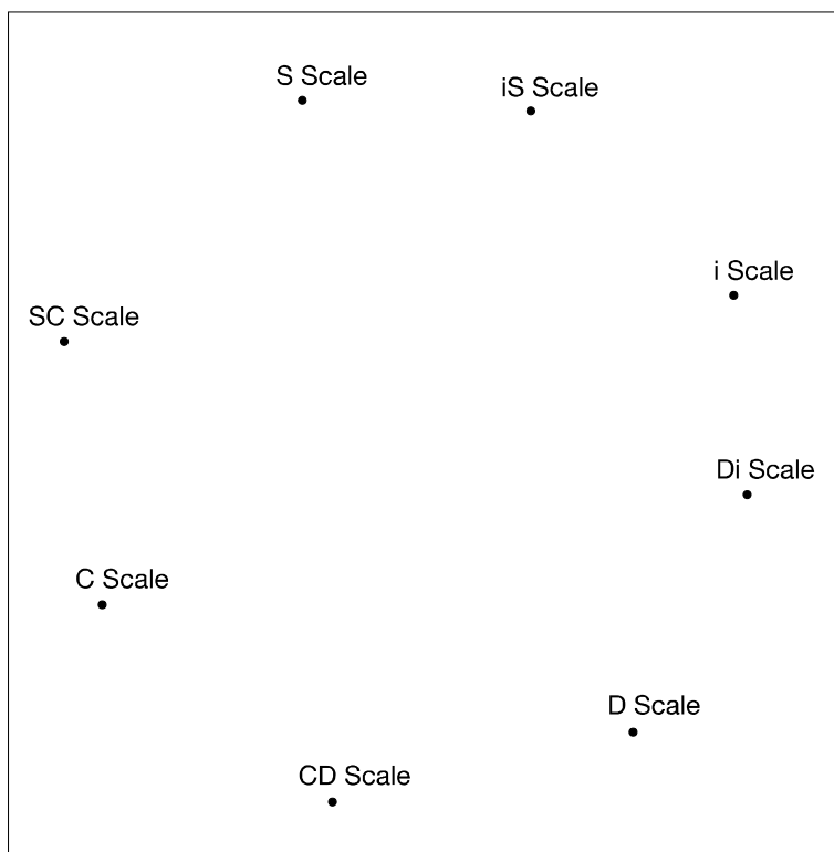
Figure 4. MDS Two-Dimensional Solution
